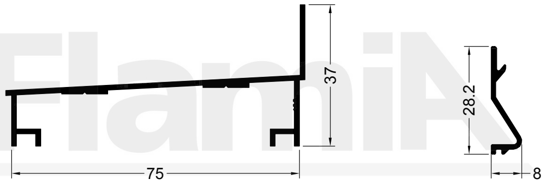
11157 0.564 Kg/m GUILLOTINA MARCO UMBRAL/DINTEL
