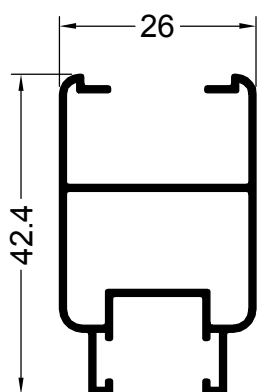
12586 0.415 Kg/m
