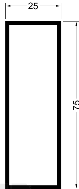
17033 0.836 Kg/m
