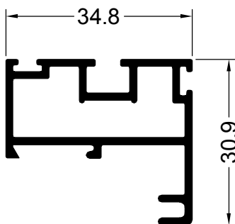
11155 0.538 Kg/m GUILLOTINA HOJA JAMBA
