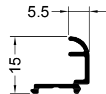
12707 0.112 Kg/m GUILLOTINA CONTRAVIDRIO CURVO 5.5 mm.
