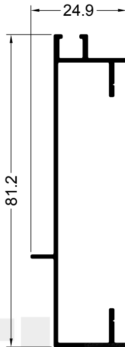
12795 0.426 Kg/m
