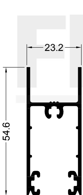
99248 0.603 Kg/m CORREDIZA HOJA JAMBA DVH
