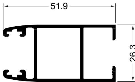
99203 0.632 Kg/m CORREDIZA HOJA JAMBA V. SIMPLE
