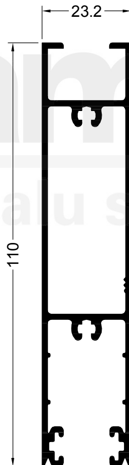
99209 1.250 Kg/m CORREDIZA HOJA UMBRAL V. SIMPLE
