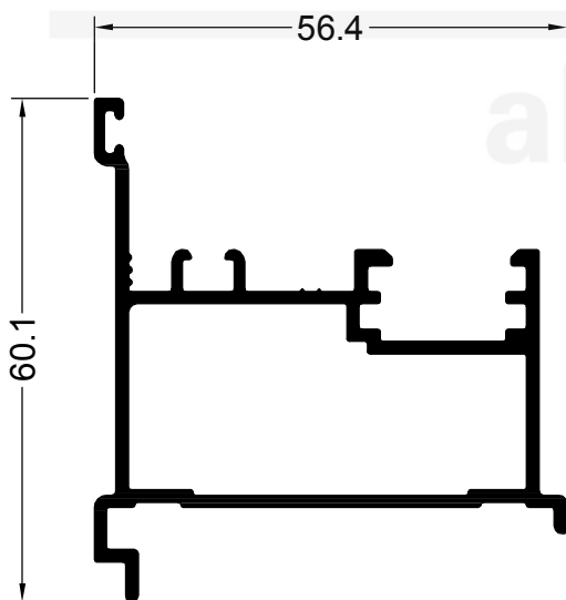
12543 0.965 Kg/m
