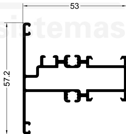
12509 0.929 Kg/m
