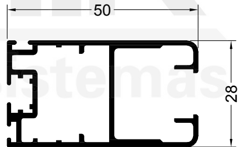
13152 0.729 Kg/m GUILLOTINA HOJA V. SIMPLE
