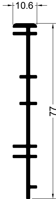
12708 0.522 Kg/m ACOPLE 75/60 mm. S/PREMARCO
