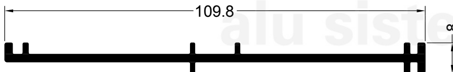
13925 0.707 Kg/m ACOPLE 105/60 mm.
