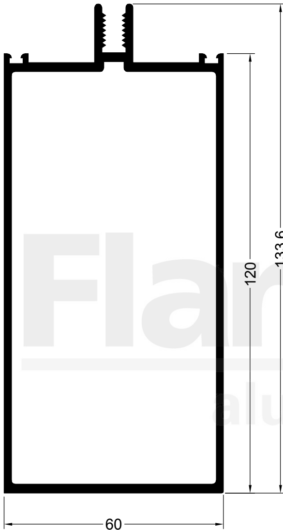
12116 2.265 Kg/m COLUMNA 134 mm.
