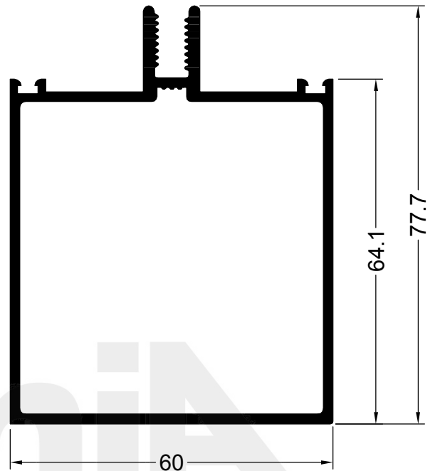
11973 1.377 Kg/m COLUMNA 78 mm.
