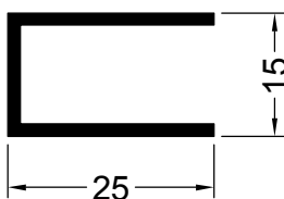
12360 0.234 Kg/m COMPLEMENTO 25 x 15 x 1.5 mm.
