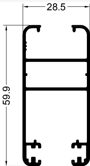
12580 0.747 Kg/m CORREDIZA HOJA V. SIMPLE
