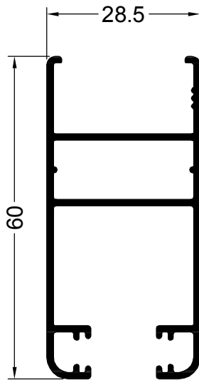
13334 0.680 Kg/m CORREDIZA HOJA JAMBA DVH
