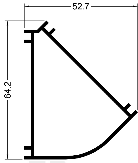
12513 0.752 Kg/m ACOPLE 135°
