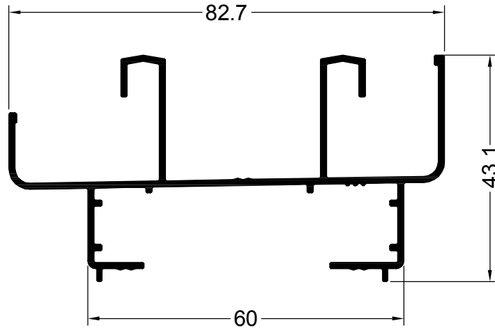
13030 0.839 Kg/m CORREDIZA MARCO
