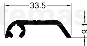
13686 0.268 Kg/m UMBRAL TRANSITABLE PISO
