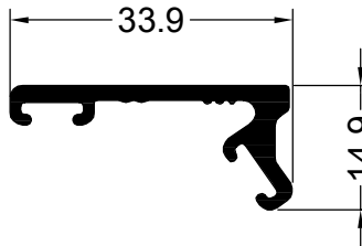
13685 0.314 Kg/m UMBRAL TRANSITABLE HOJA
