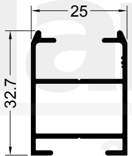
11774 0.399 Kg/m POSTIGON HOJA 33 mm.
