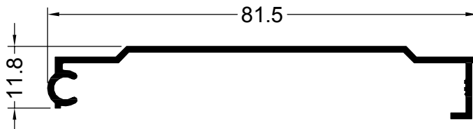
11683 0.382 Kg/m CORREDIZA TAPACINTA 81.5 mm.
