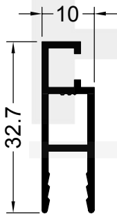
10842 0.257 Kg/m CORREDIZA MOSQUITERO HOJA
