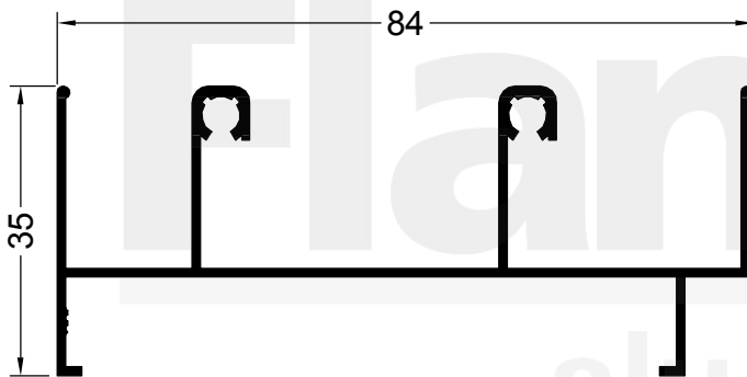
11681 0.691 Kg/m CORREDIZA MARCO 90° UMBRAL/DINTEL
