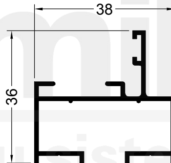
11775 0.426 Kg/m POSTIGON MARCO 38 mm.
