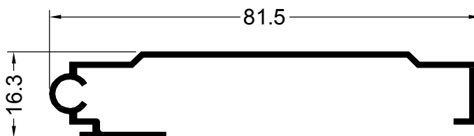
11682 0.370 Kg/m CORREDIZA TAPACINTA 81.5 mm. FALSO
